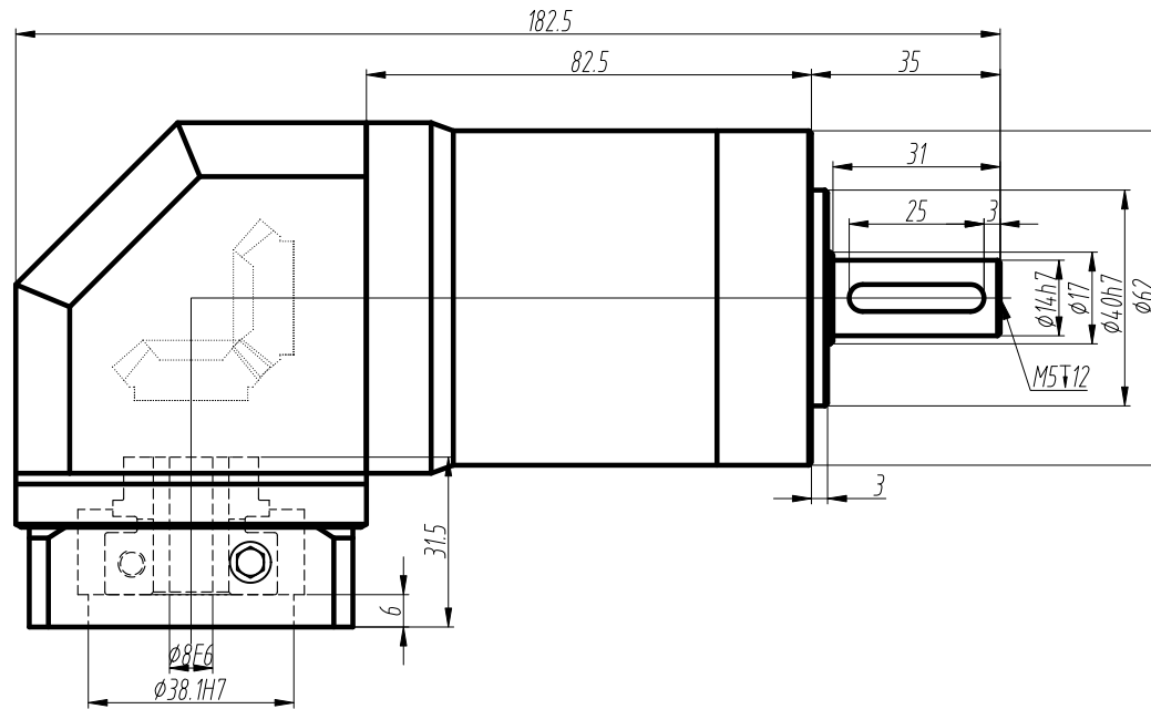
标准轴 Standard output shaft
